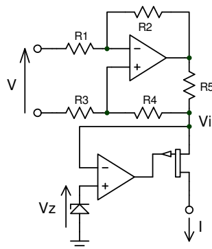
Figure 8: Current source with cascode stage.
