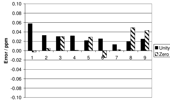
Figure 11: Zero and unity error test results.
