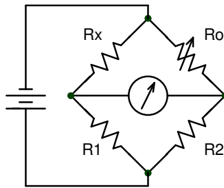
Figure 1: Wheatstone bridge.
