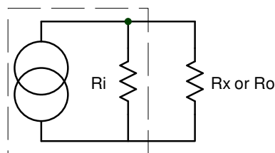
Figure 5: Effect of current source output impedance.
