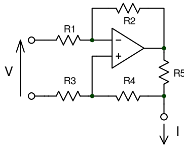
Figure 7: Basic current source.
