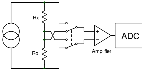
Figure 3: Potentiometric resistance instrument.
