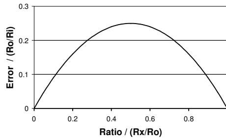
Figure 6: Error from current source impedance.
