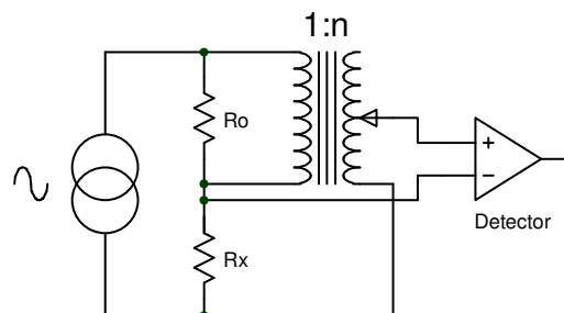
Figure 2: AC ratio transformer bridge.
