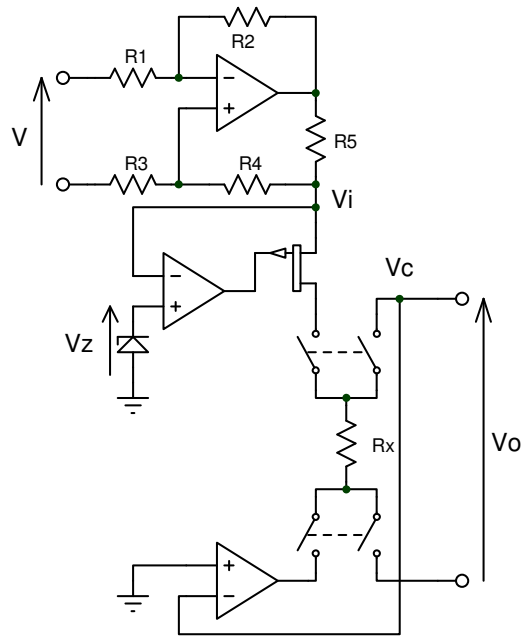
Figure 9: Guarded current source.
