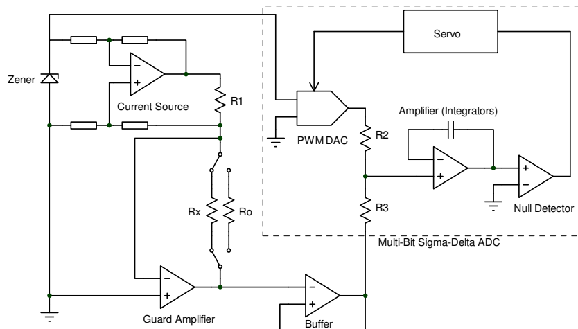
Figure 10: microK bridge measurement system.
