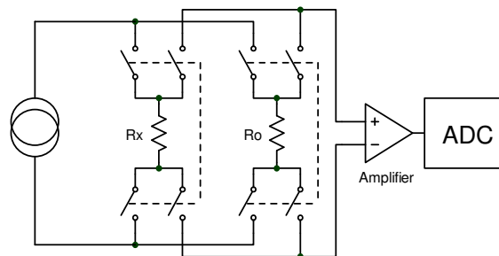
Figure 4: Substitution topology.
